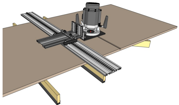
Using the Super Smart Routing Kit* and EZ SMART Tracksaw System*
